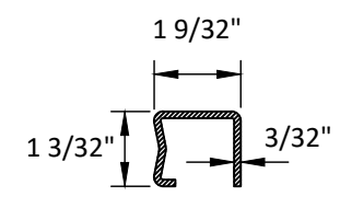
⑧ REINFORCEMENT
