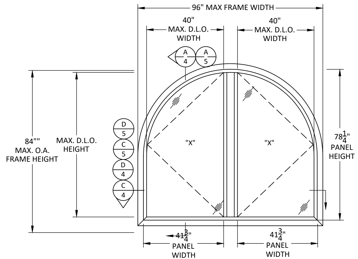
ELEVATION INSWING OR OUTSWING
