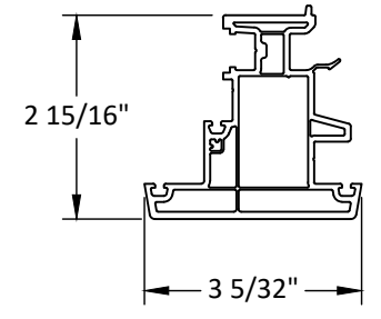
⑤ MULLION
