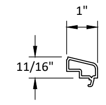
② I.G. GLAZING BEAD
