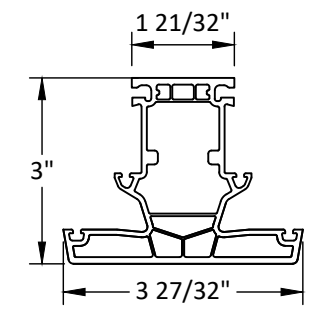
⑩ MULLION
