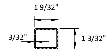
⑦ REINFORCEMENT
