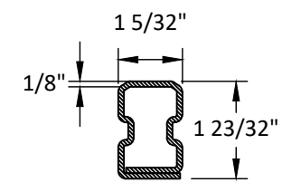
⑨ REINFORCEMENT
