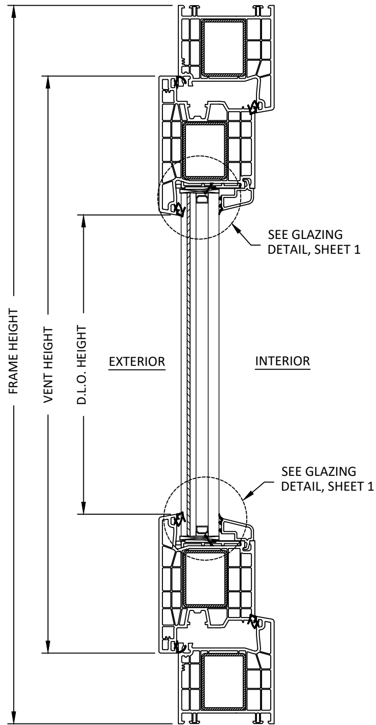
A 4 VERTICAL SECTION OPERABLE WINDOW
