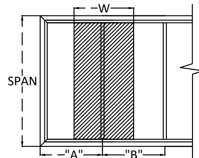
ANCHOR LAYOUT THROUGH FRAME
