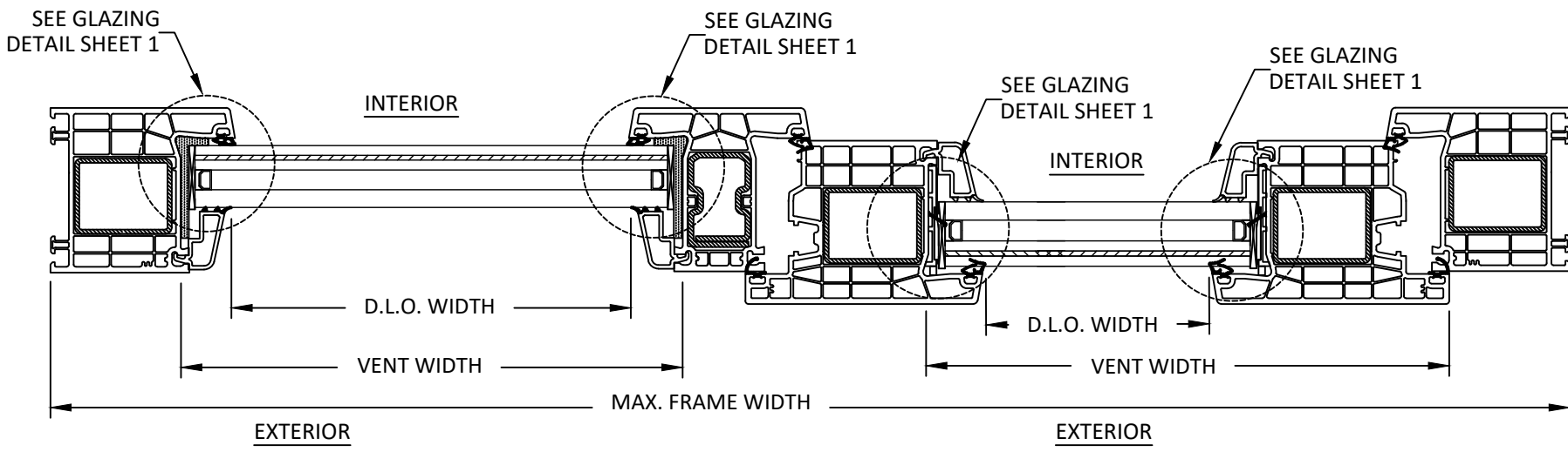
C 5 HORIZONTAL SECTION OPERABLE FIXED WINDOW
