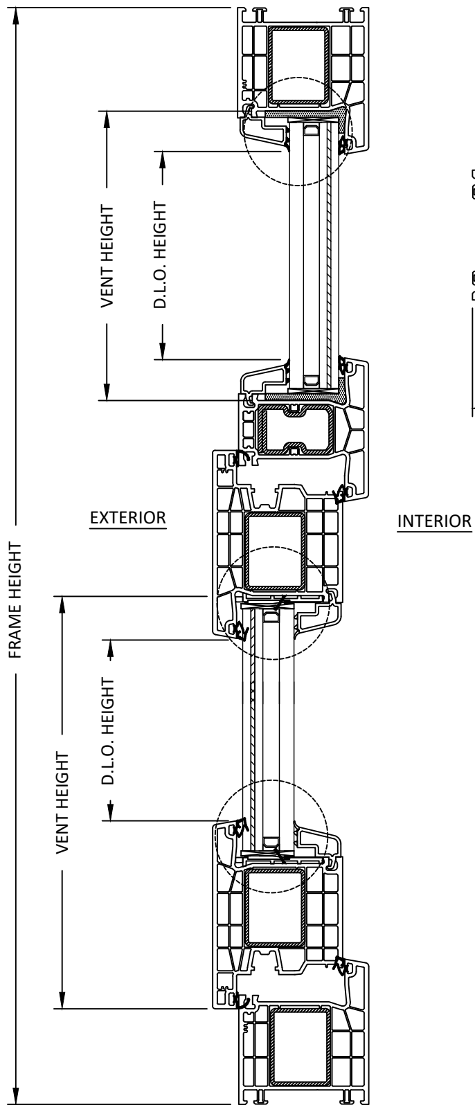
A 5 VERTICAL SECTION OPERABLE FIXED WINDOW
