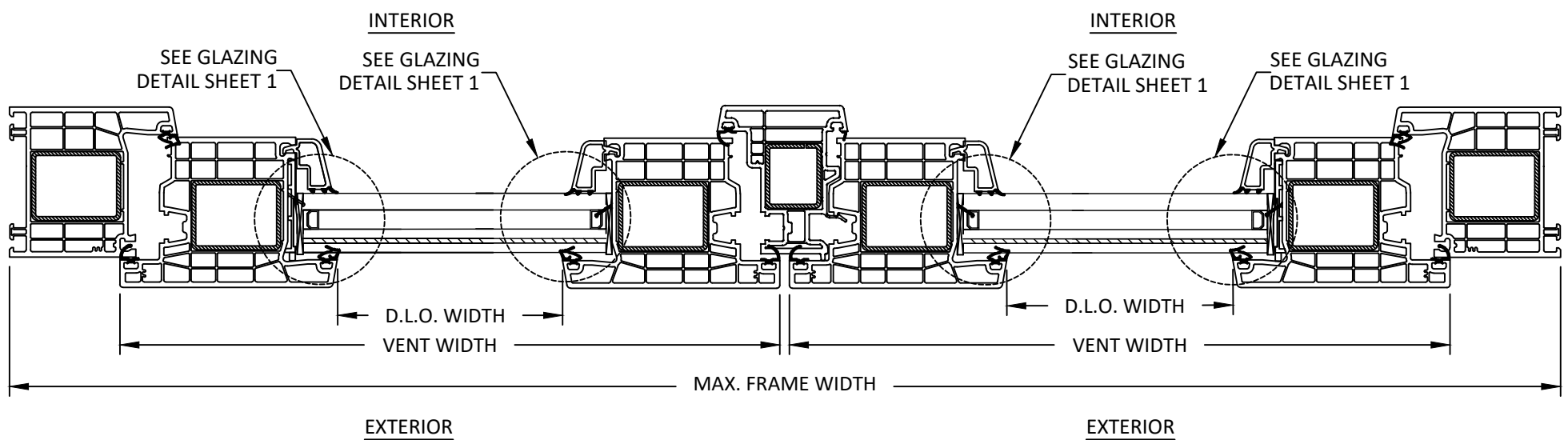
C 4 HORIZONTAL SECTION OPERABLE TWIN WINDOW
