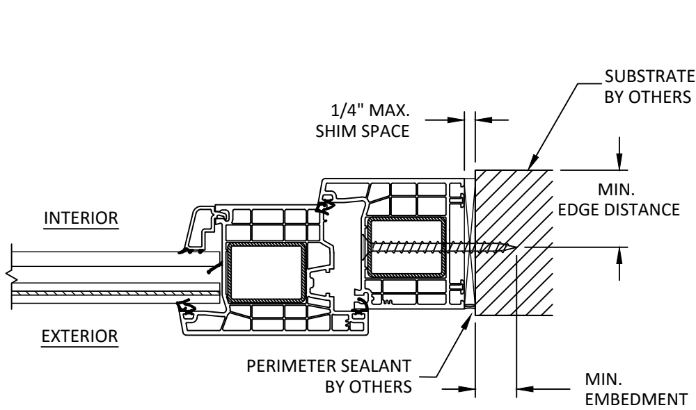
A 6 HORIZONTAL SECTION THROUGH FRAME (JAMB)
