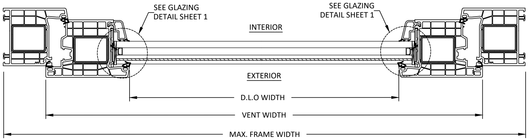
B 4 HORIZONTAL SECTION OPERABLE WINDOW
