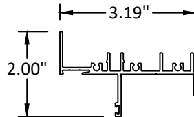
⑯ FRAME HEAD
