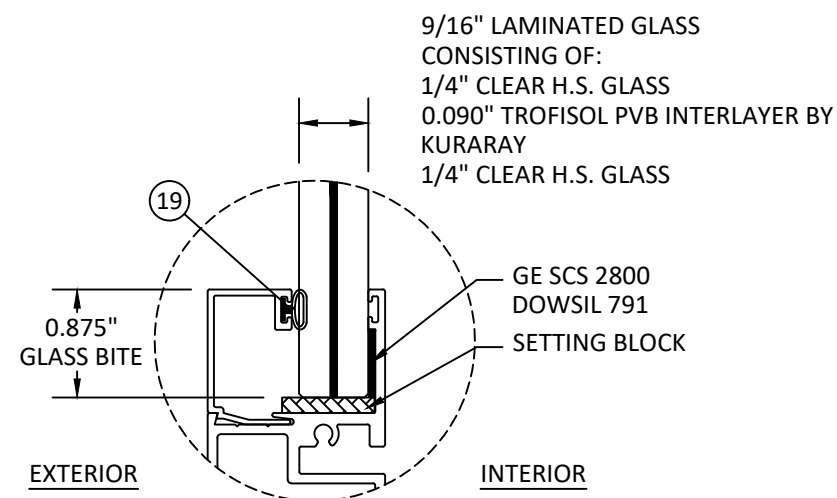
GLAZING DETAIL G3
