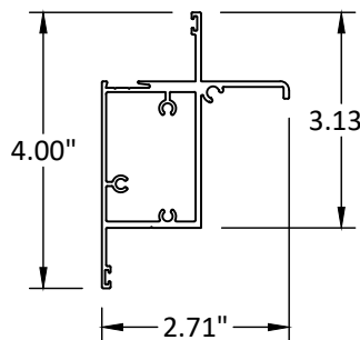
④ SASH BOTTOM RAIL
