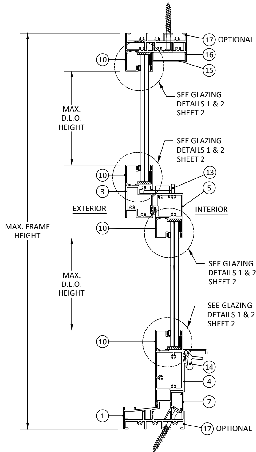
A 6 VERTICAL SECTION SINGLE HUNG WINDOW
