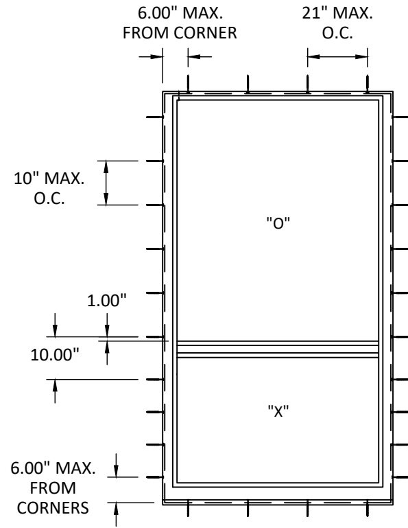
ELEVATION SINGLE HUNG WINDOW - ORIEL
