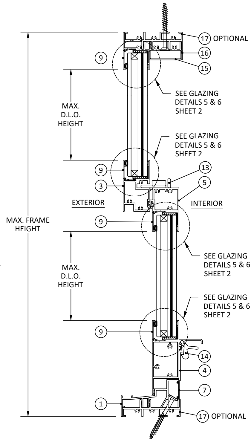
C 6 VERTICAL SECTION SINGLE HUNG WINDOW
