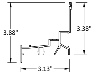
① SILL
