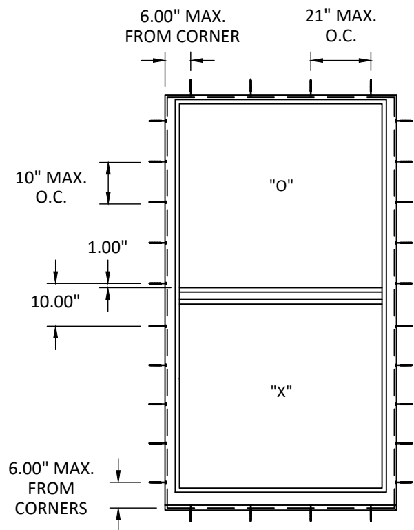
ELEVATION SINGLE HUNG WINDOW - EQUAL LITES
