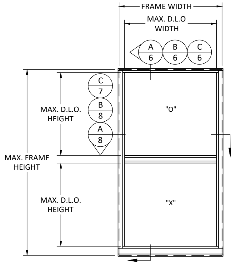
ELEVATION SINGLE HUNG WINDOW - EQUAL LITES
