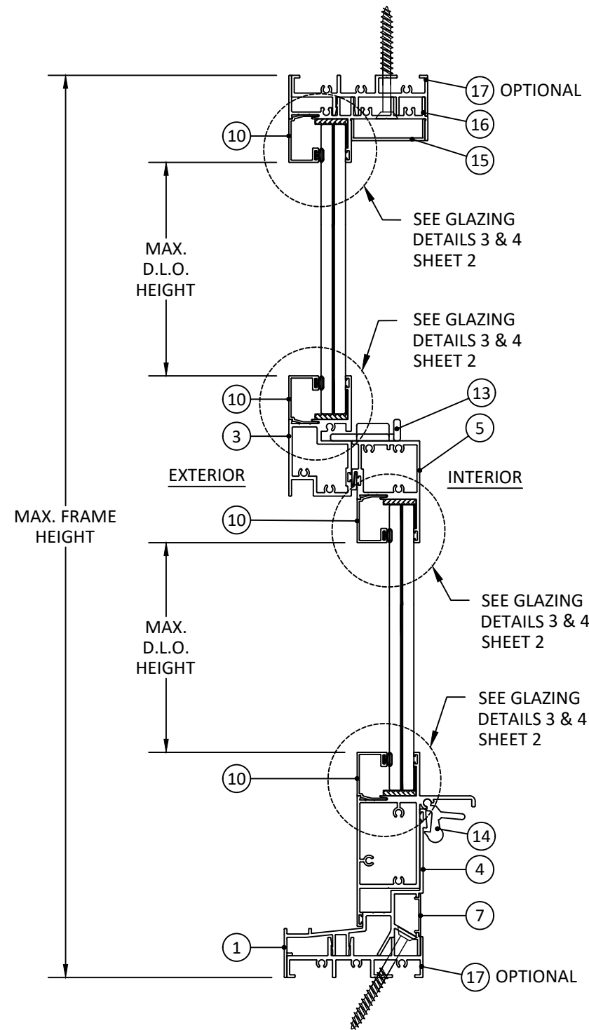
B 6 VERTICAL SECTION SINGLE HUNG WINDOW
