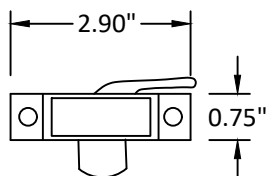
⑬ SASH LOCK
