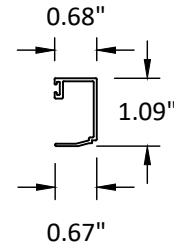
⑩ GLAZING LAMI
