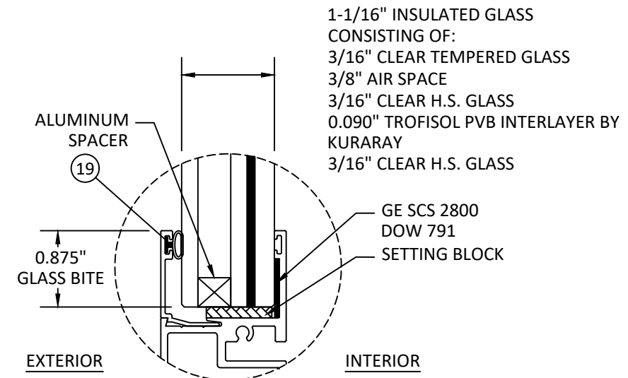
GLAZING DETAIL G5
