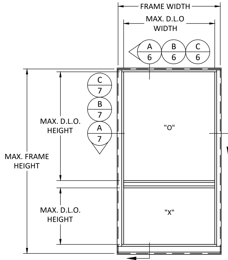
ELEVATION SINGLE HUNG WINDOW - ORIEL
