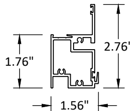
③ MEETING RAIL
