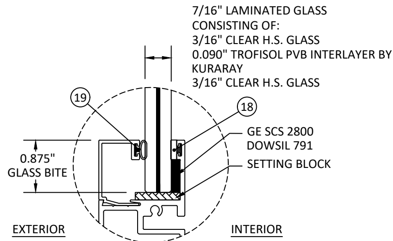
GLAZING DETAIL G1
