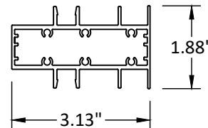
⑪ EQUAL LEG ADAPTER
