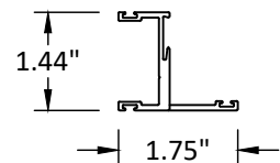
⑥ SASH STILE
