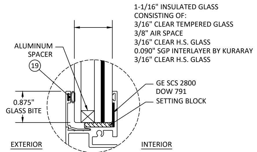
GLAZING DETAIL G6
