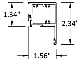
⑤ SASH TOP RAIL
