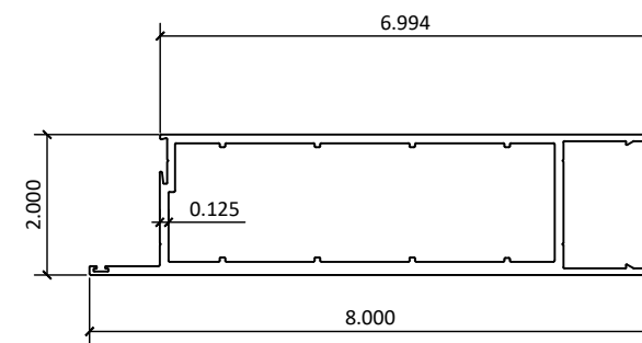
12 600-13 - BOTTOM RAIL 8"
