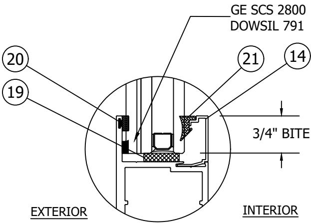
GLAZING DETAIL 3
