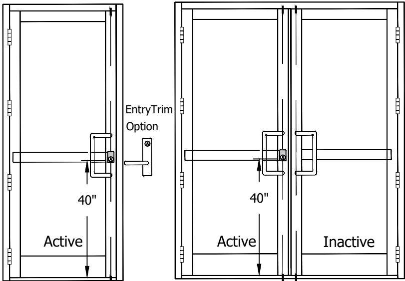
LOCK OPTION #5: *ONLY FOR DOORS WITH HEIGHT ≤ 96"
