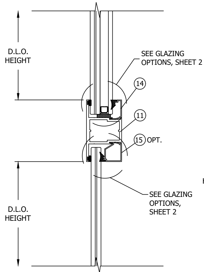
B 7 VERTICAL SECTION MEETING RAIL OPTIONAL
