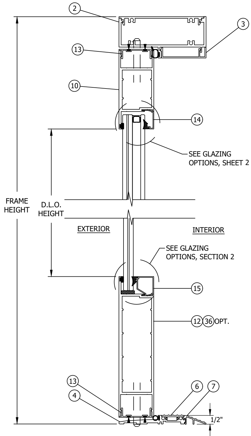
A 7 VERTICAL SECTION HEAD - ADA SILL
