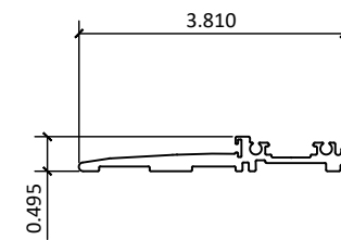
4 600-04 - THRESHOLD
