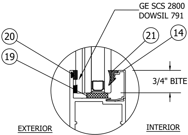
GLAZING DETAIL 4
