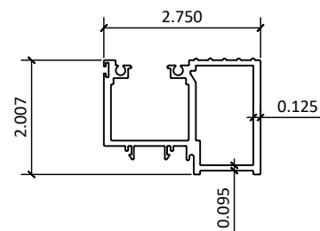
5 600-05 - THRESHOLD ADAPTER
