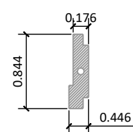
16 600-18 - ASTRAGAL REINFORCEMENT
