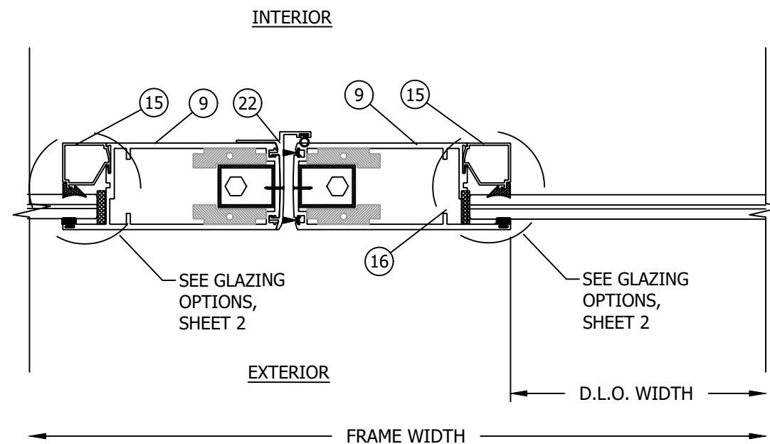
D HORIZONTAL SECTION 9 STILE REINFORCED ADAMS RITE 3 POINT LOCK
