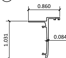
19 600-14 - ASTRAGAL ADAPTER
