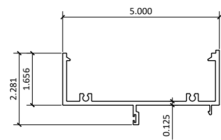
2 600-02 - HEAD
