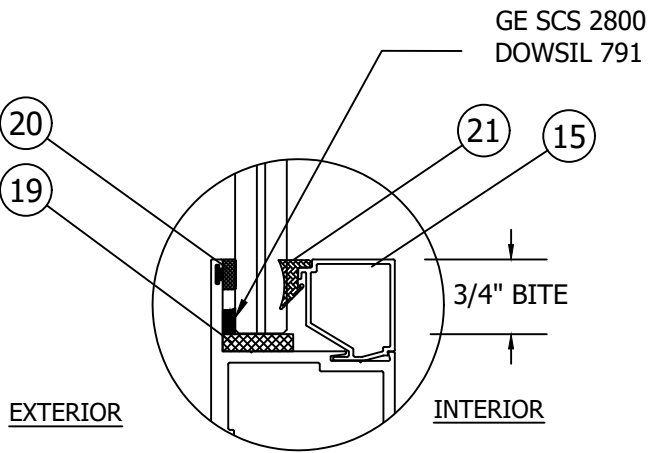
GLAZING DETAIL 2
