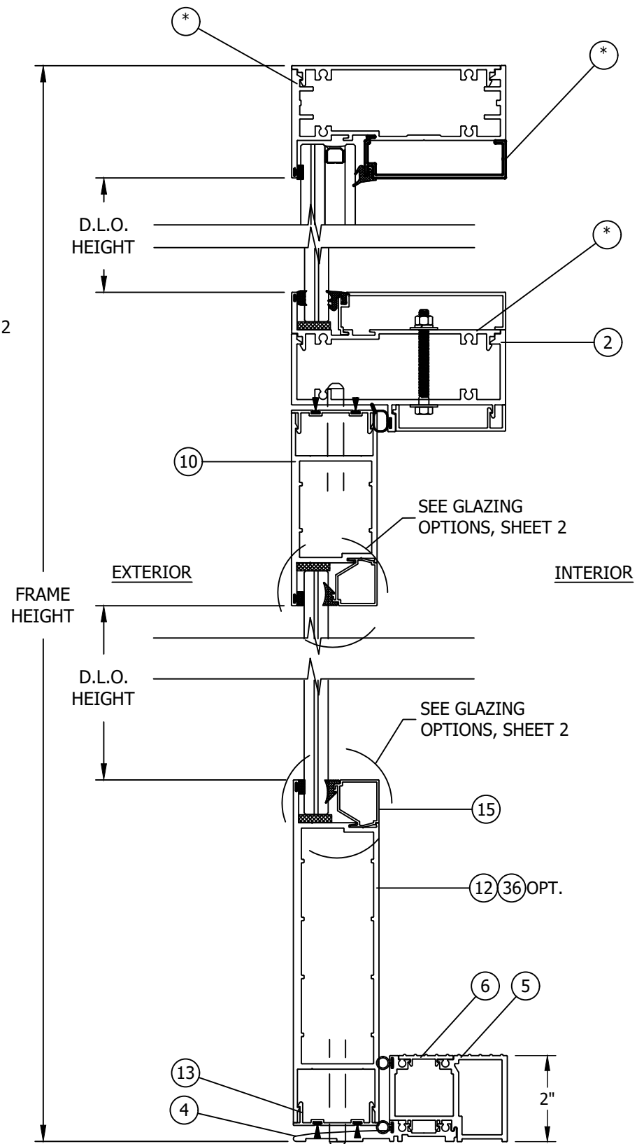
C 7 VERTICAL SECTION HEAD W/TRANSOM- WATER SILL
