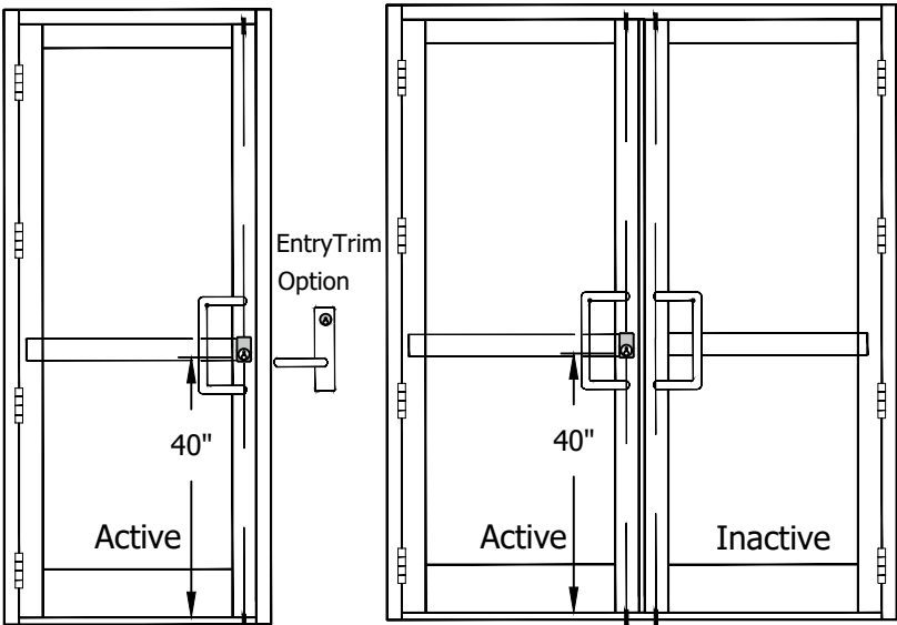
LOCK OPTION #4:
