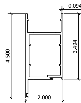
10 600-11 - TOP RAIL
