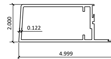
12 600-13 - BOTTOM RAIL 8"
