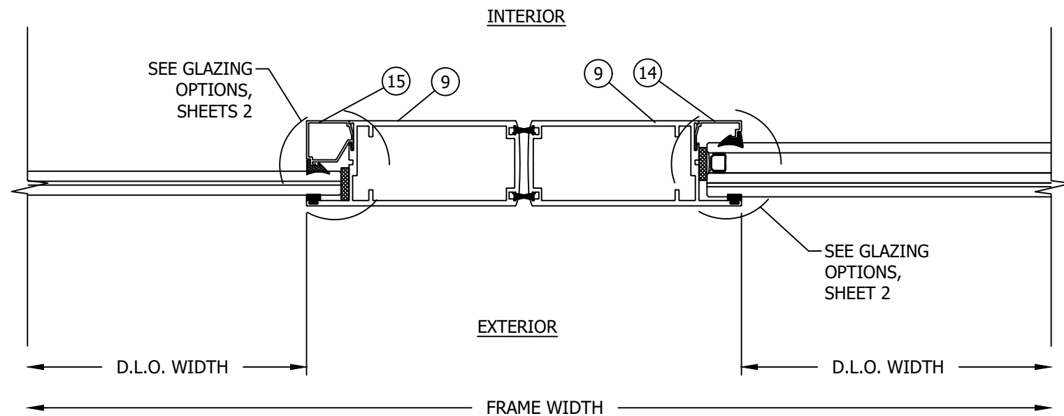
A HORIZONTAL SECTION 9 ASTRAGAL WITHOUT REINFORCEMENT DOOR HEIGHT < 96"
