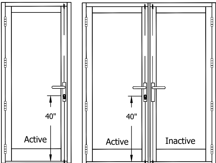
LOCK OPTION #2:
