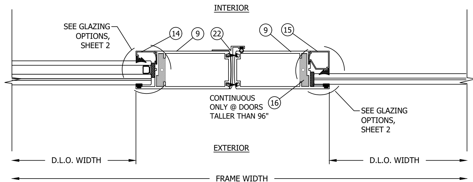
B HORIZONTAL SECTION 9 ASTRAGAL W/T REINFORCEMENT DOOR HEIGHT ≥ 96"
