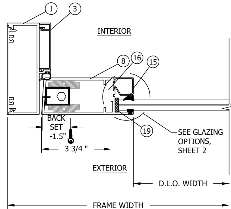
C HORIZONTAL SECTION 9 STILE REINFORCED ADAMS RITE 3 POINT LOCK
