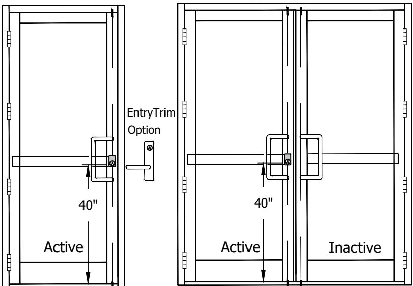
LOCK OPTION #3:
